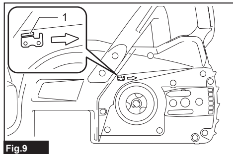
► 1. Mark on chain saw body
